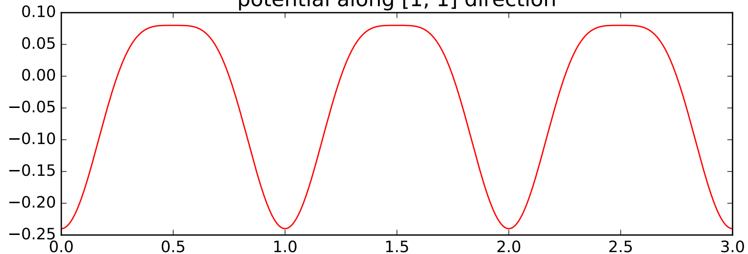
potential along [1, 1] direction
